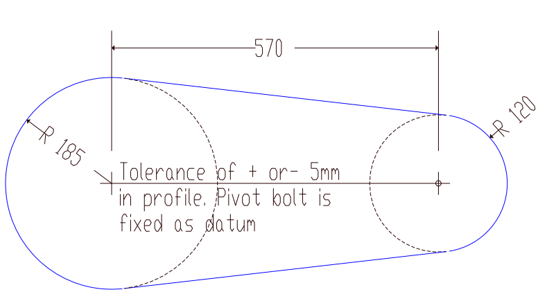
Rudder (Maximum thickness 22mm)
